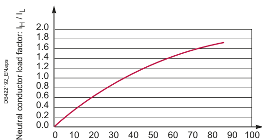
Fig. E57 Neutral conductor load factor as a function of the 3rd harmonic level.
