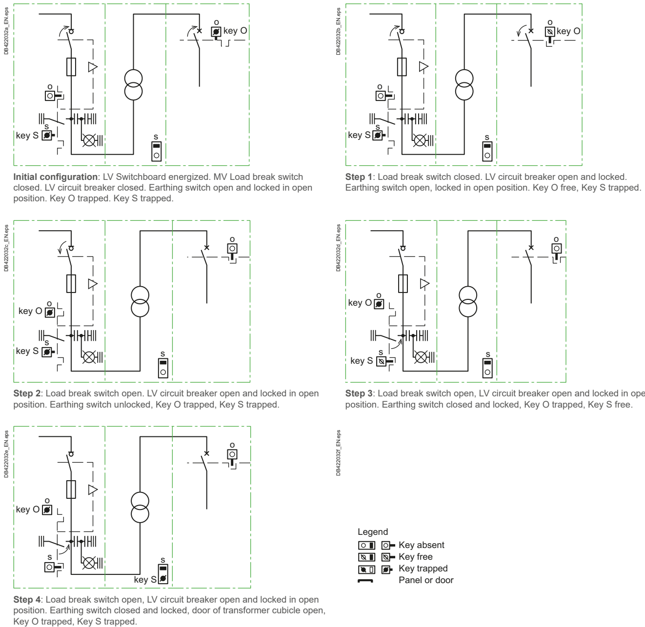
Fig. B30 Example of MV/LV interlocking system
