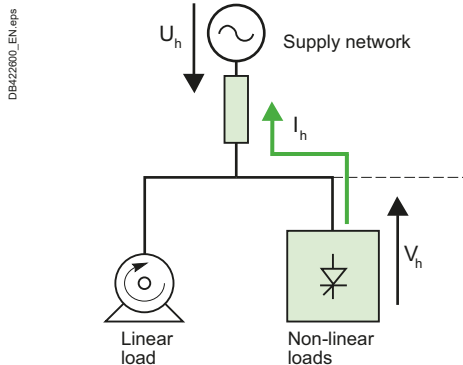
Fig. L29 Simplified circuit diagram
