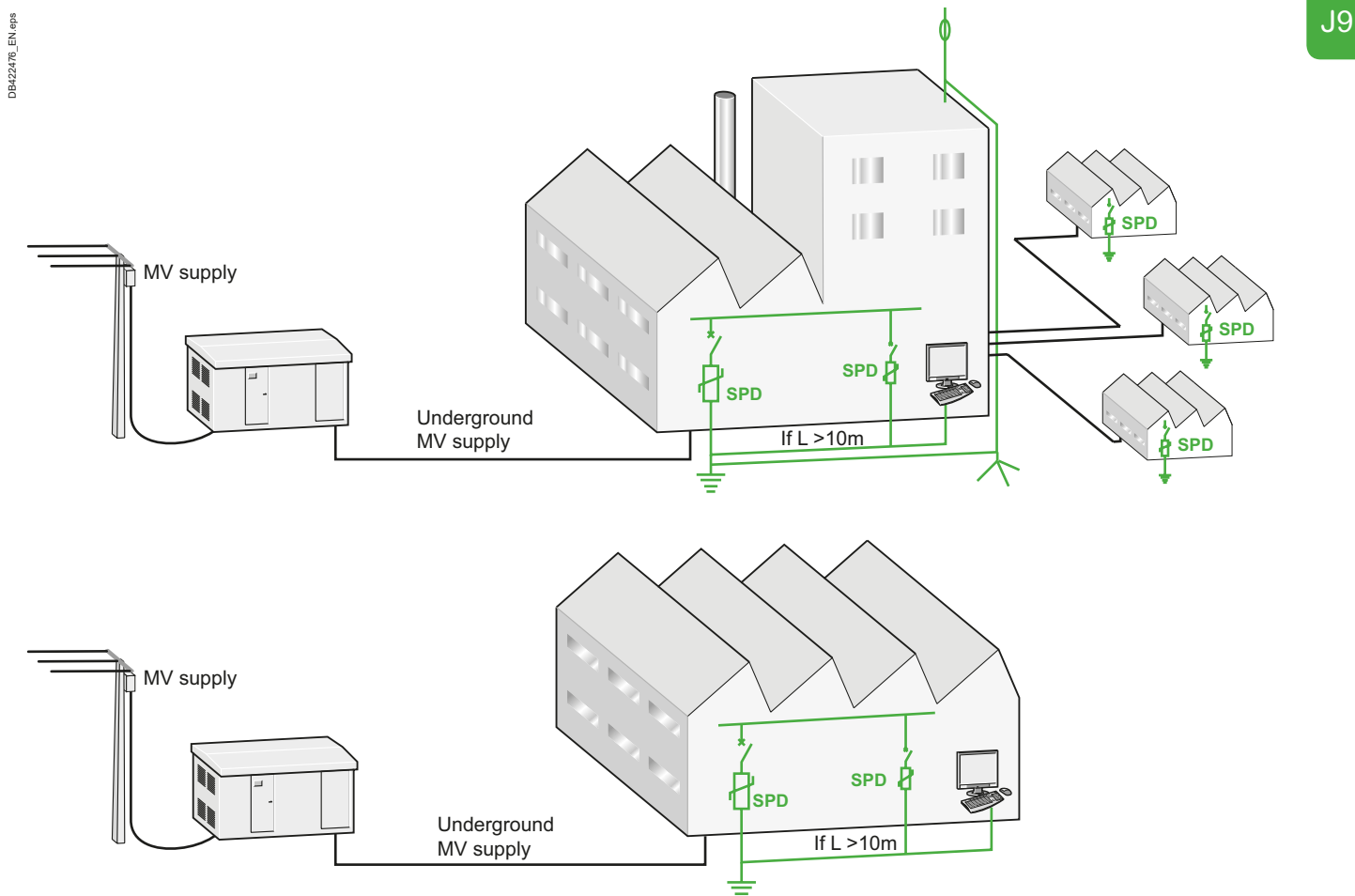
Fig. J16 Example of protection of a large-scale electrical installation
