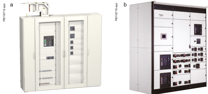
Fig. E27 [a] A main LV switchboard - MLVS - (Prisma P) with incoming circuits in the form of busways; [b] ALV motor control centre - MCC - (Okken)
