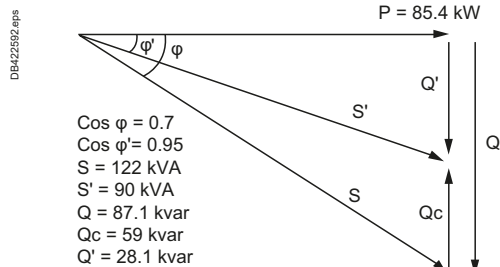
Fig. L17 Reduction of declared maximum kVA by power-factor improvement
