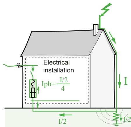
Fig. J30 Basic example of balanced limp current distribution in 3 phase system
