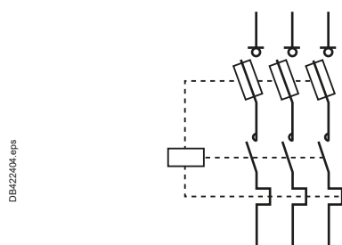
Fig. H18 Symbol for a fuse-switch disconnect + disconnector
